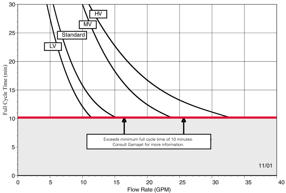
Gamajet Aseptic 6 - Flow Rate vs. Typical Full Cycle Time
