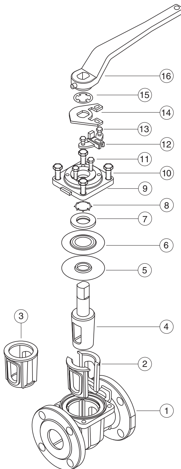
FIGURE II-1 Typical Assembly of Mach 1
